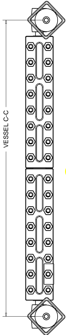
Vessel Connection Behind Gage Face Fig. 4-1
