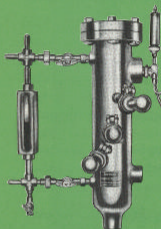
Lowwater Alarm with Triple Valve Assembly, Gauge and Gauge Cocks
