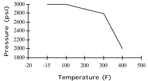
Fig. 1 SFI Pressure and Temperature Rating
